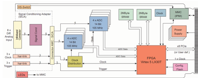
Figure 3. Block diagram of TAMC900
