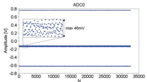
Figure 9. Example ADC0 laboratory readout
