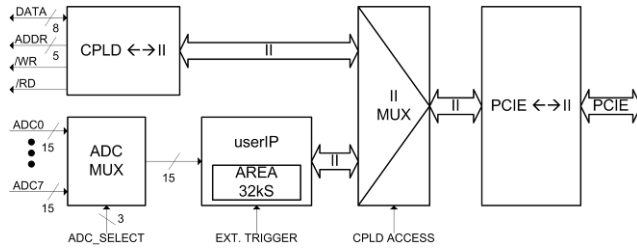
Figure 6. Block diagram of TAMC900 firmware
