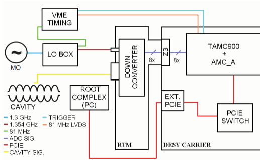
Figure 10. Block diagram of ACC6 test setup
