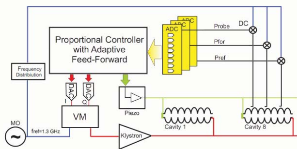
Figure 1. Block diagram of LLRF controller
