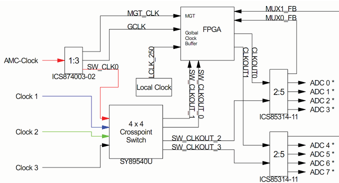
Figure 4. TAMC900 clocks distribution
