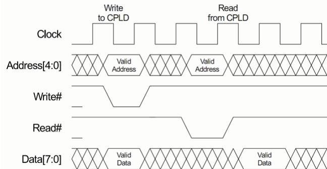
Figure 5. FPGA to CPLD interface
