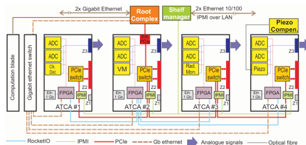
Figure 2. Block diagram of ATCA based controller
