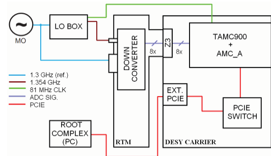
Figure 7. Block diagram of laboratory test setup
